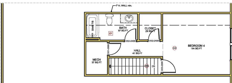
SECOND FLOOR
